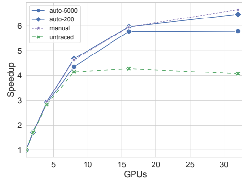
Figure 8. Strong scaling of FlexFlow on Eos.
